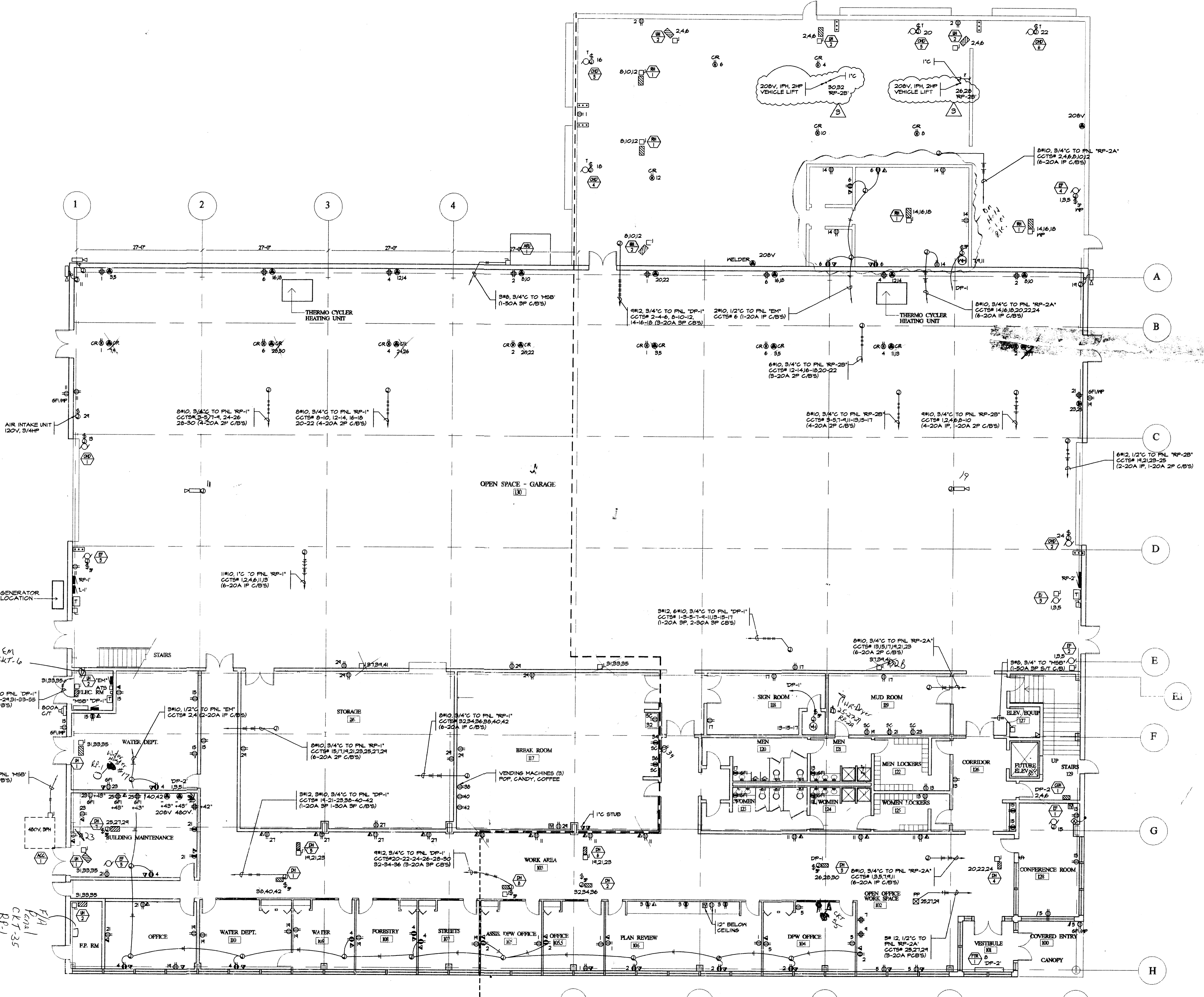
GROUND POWER FLOOR PLAN SCALE 1/8" = 1'-0"
